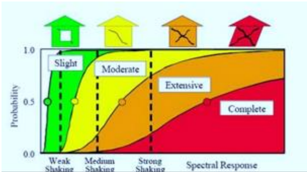
Figure 3-3, A typical fragility curve
